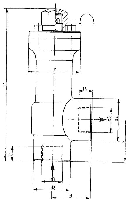
dimensional drawing
