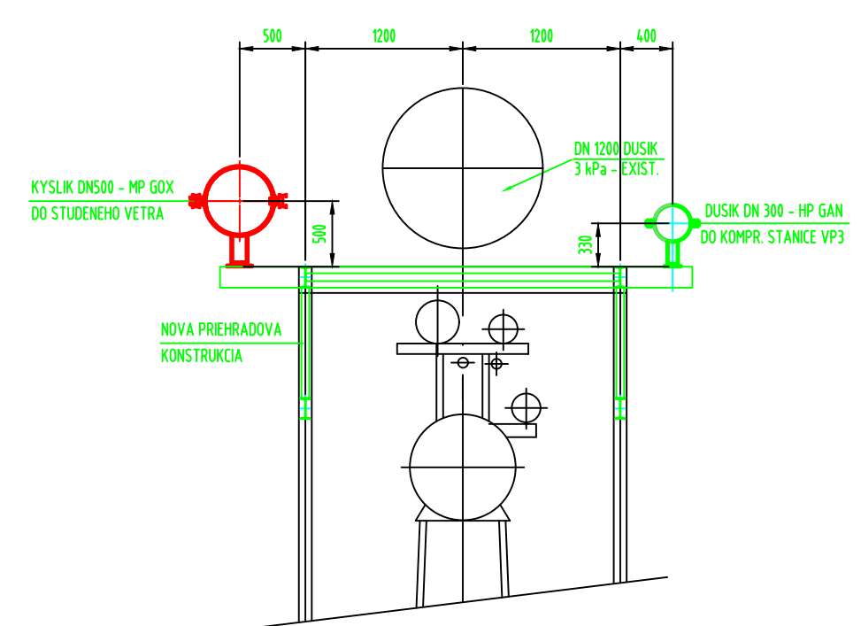
CHARAKTERISTICKÝ REZ ULOŽENIA POTRUBIA TYPICAL SECTION FOR PIPE SUPPORT
